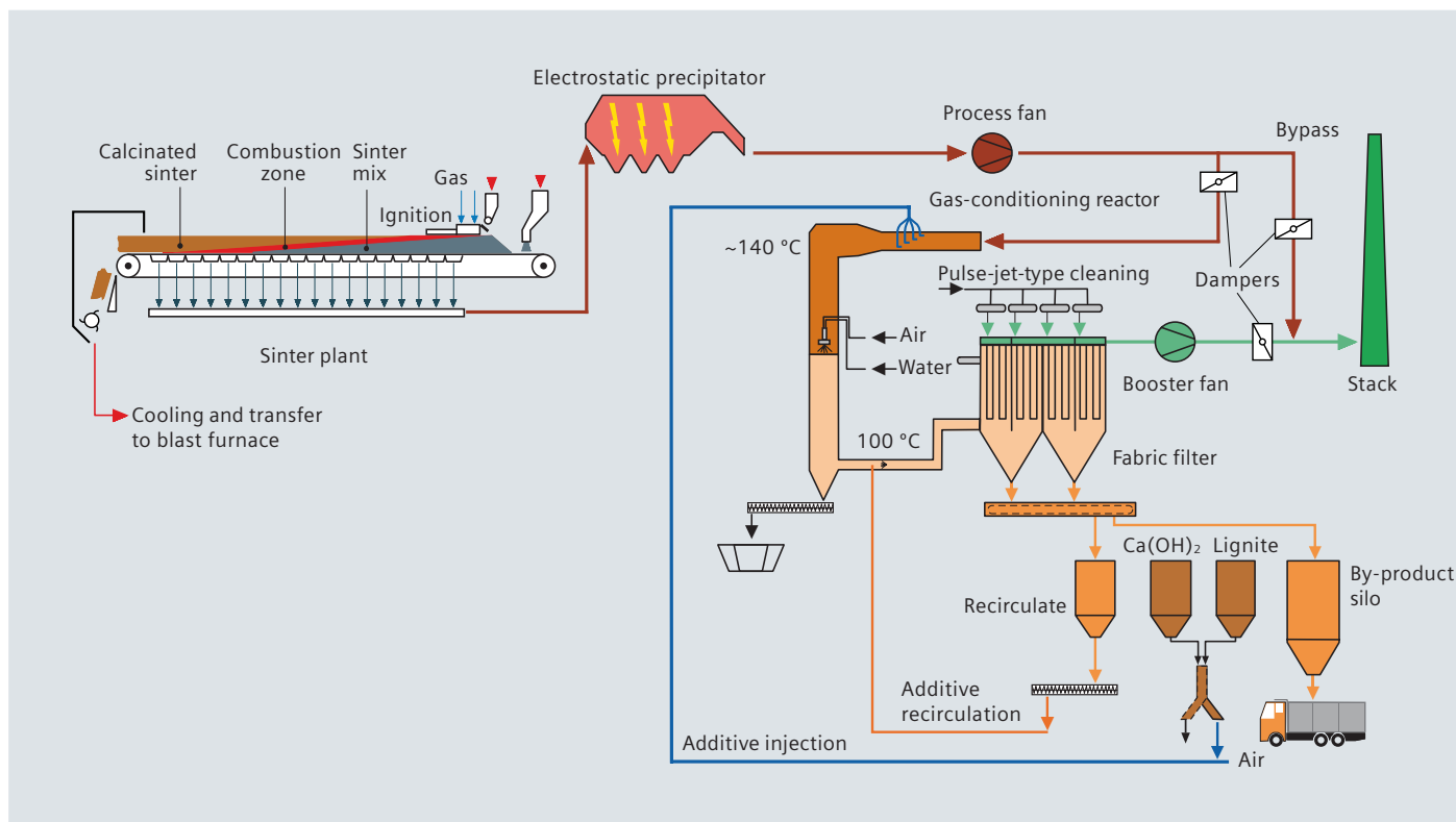
Principal process flow sheet of the SIMETAL CIS MEROS® plant
